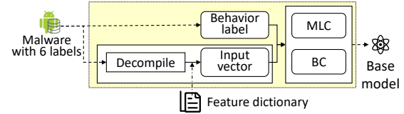
Fig. 3: Base MLC model construction with labeled dataset
