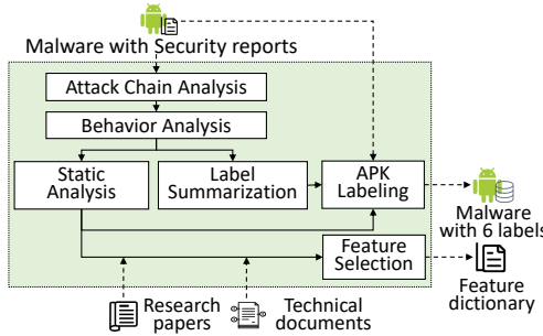
Fig. 2: Behavior analysis and data annotation
